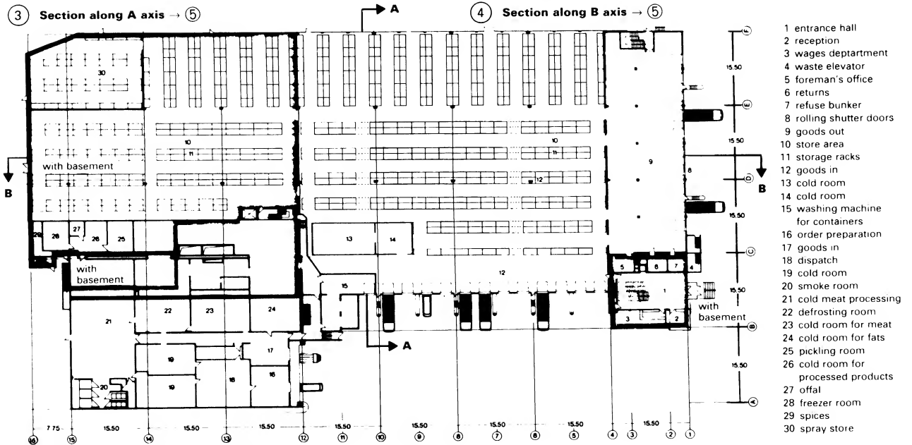
⑤ Ground floor of meat products factory
